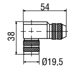
6 pin 90° female connector M16 Part No. ST C0 9131-6
